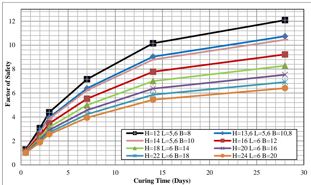
Figure 5. Graphical correlation CT and FS using modification Li and Aubertin solution
